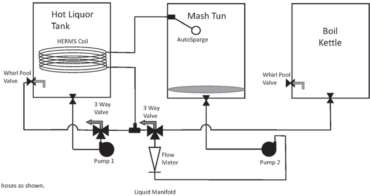
Plumbing and Hardware Schematic: 3 Vessel, Gas, HERMS
