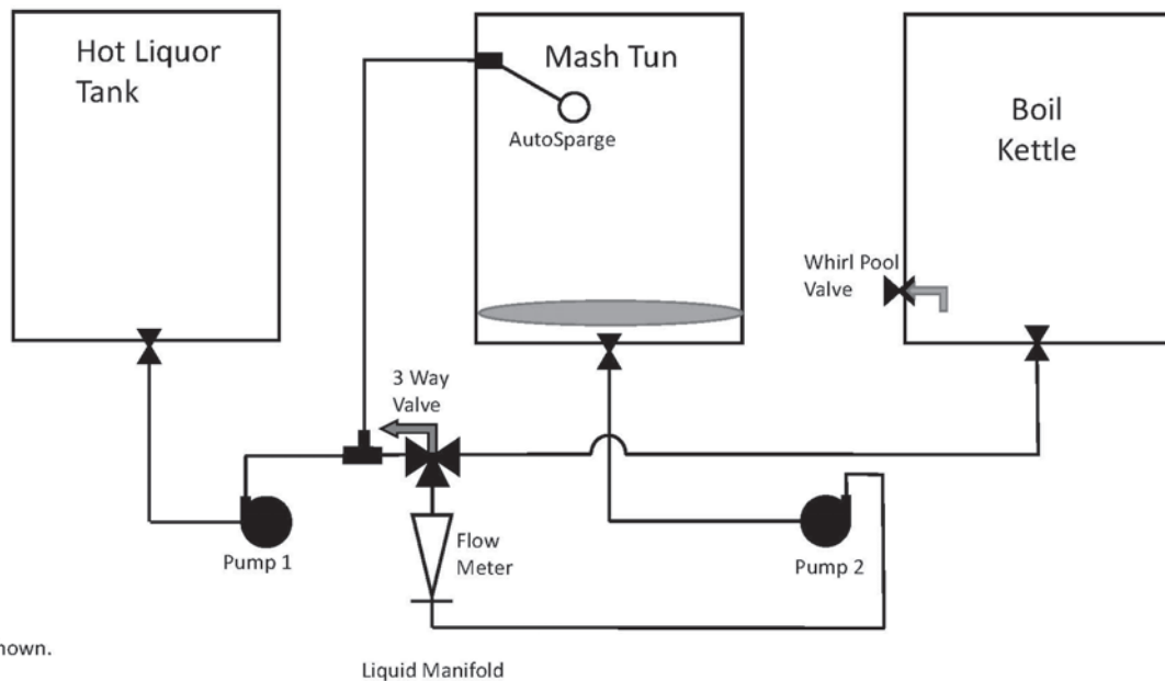
Plumbing and Hardware Schematic: 3 Vessel, Gas – Kettle RIMS
